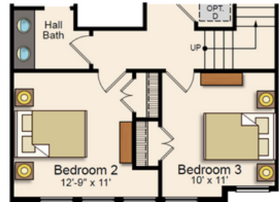
Opt. Second Floor Plan W/ Opt. Loft Stair
